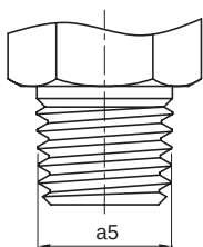
Form C (DIN 3852 Part 1&2) with sealing in tapered thread
