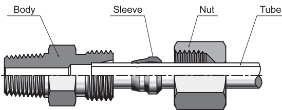
BODY, SHOULDER, SLEEVE, NUT & TUBE
