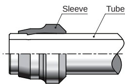
Internal ridge on Tube
