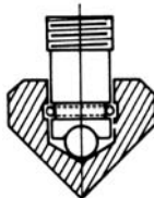
SWIVEL-TYPE BALL BEARING CONE - Ball thrust bearing in flaring cone minimizes friction, makes operation easier.
