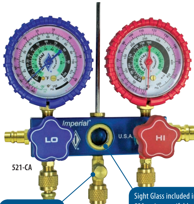
Auxiliary valve port
