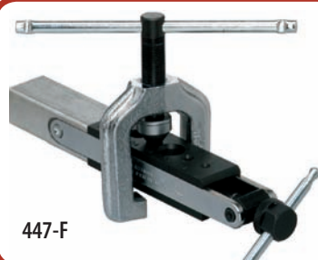
SWIVEL-TYPE BALL BEARING CONE - Ball thrust bearing in flaring cone minimizes friction, makes operation easier.
